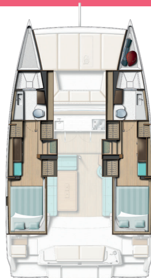
2 DOUBLE CABINS / 2 HEADS VERSION VERSION 2 CABINES DOUBLES / 2 SDB
